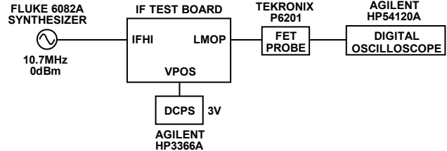
Figure 20. Test Circuit for Limiter Rise and Fall Times (Figure 10)
